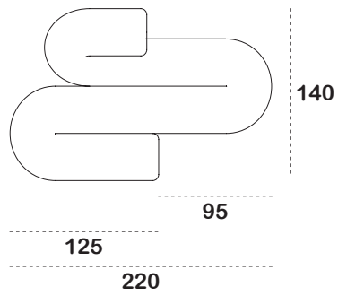
SR 220 B1C1
