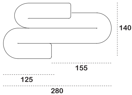
SR 280 B1C1
