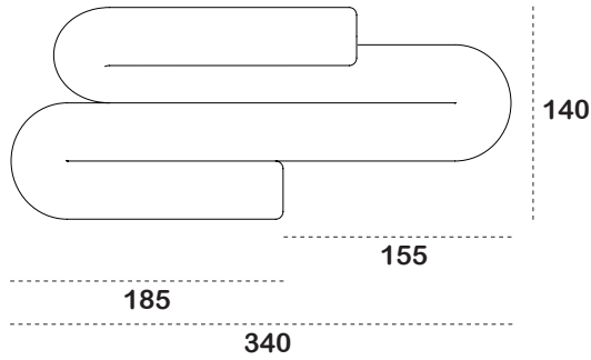
SR 340 B1C2
