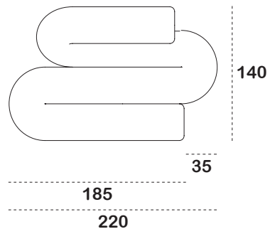
SR 220 C2
