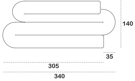
SR 340 C4
