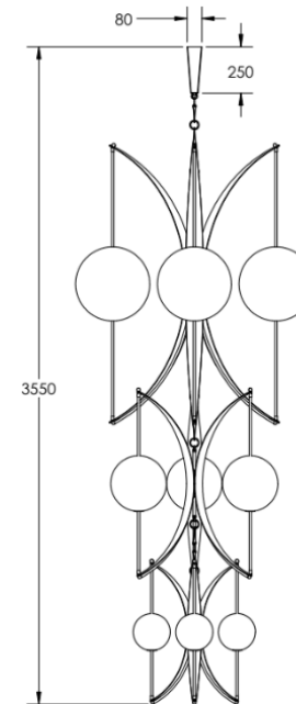
FRONT ELEVATION
