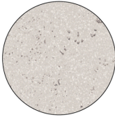
Urban Sandstone
